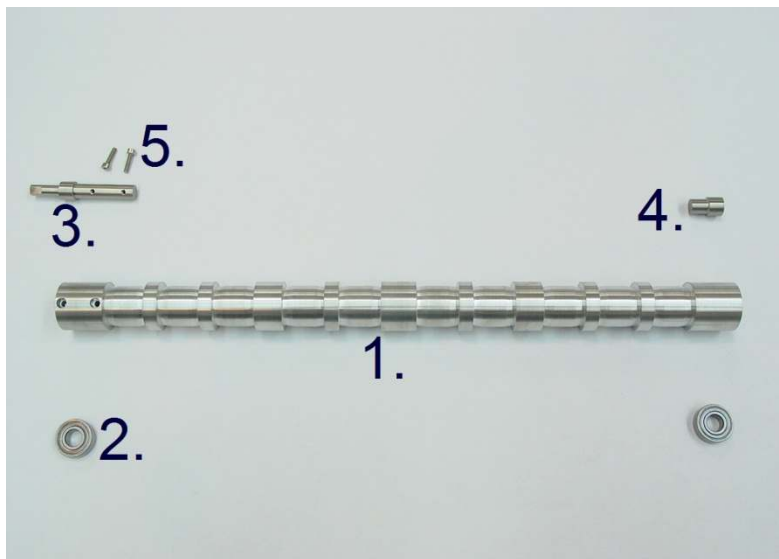
(1) SP 006 292 DRIVE ROLLER COMPLETE
