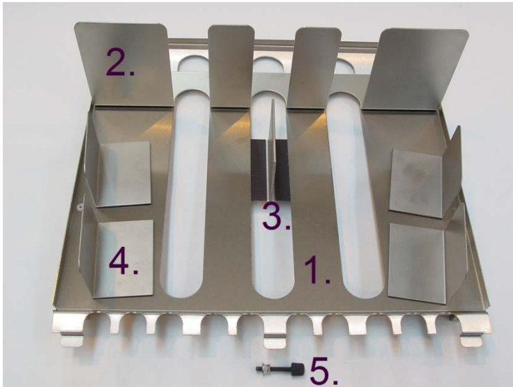
(1) SP 006 535 TRAY, STACKING, STANDARD
